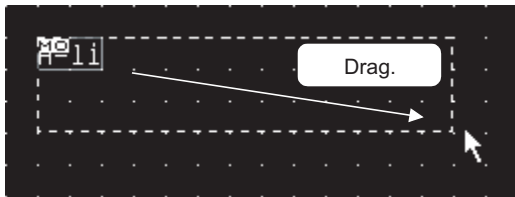
Base screen 1
