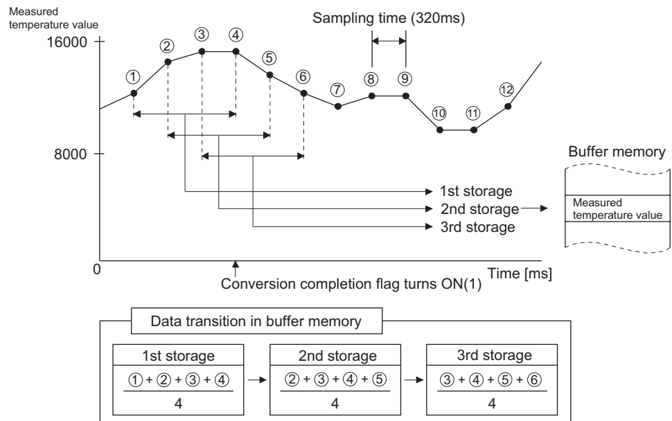
Moving average processing when setting is 4 times.
